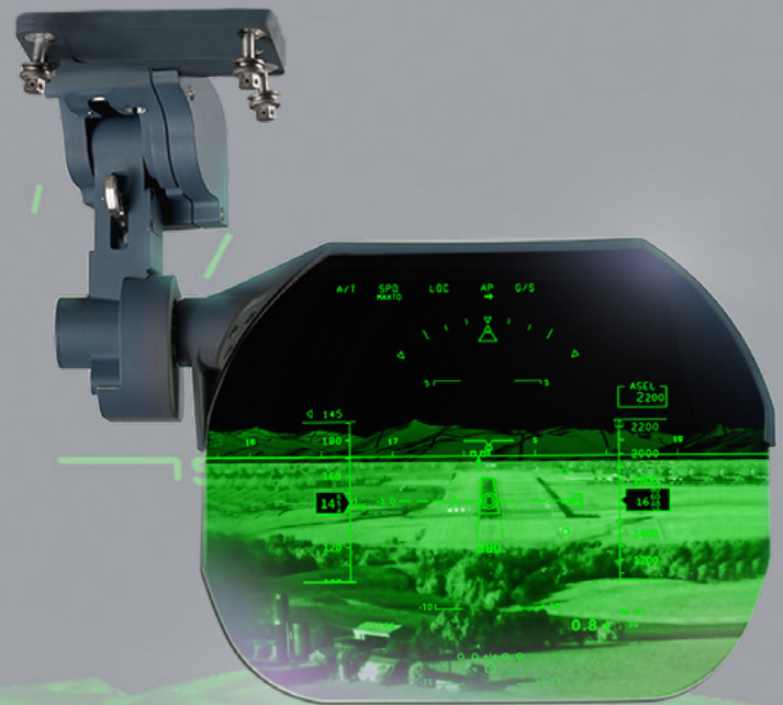
Overhead-Mounted Digital HUD
