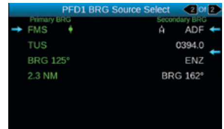
PFD BRG Source Select Page
