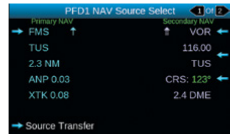
PFD Nav Source Select Page
